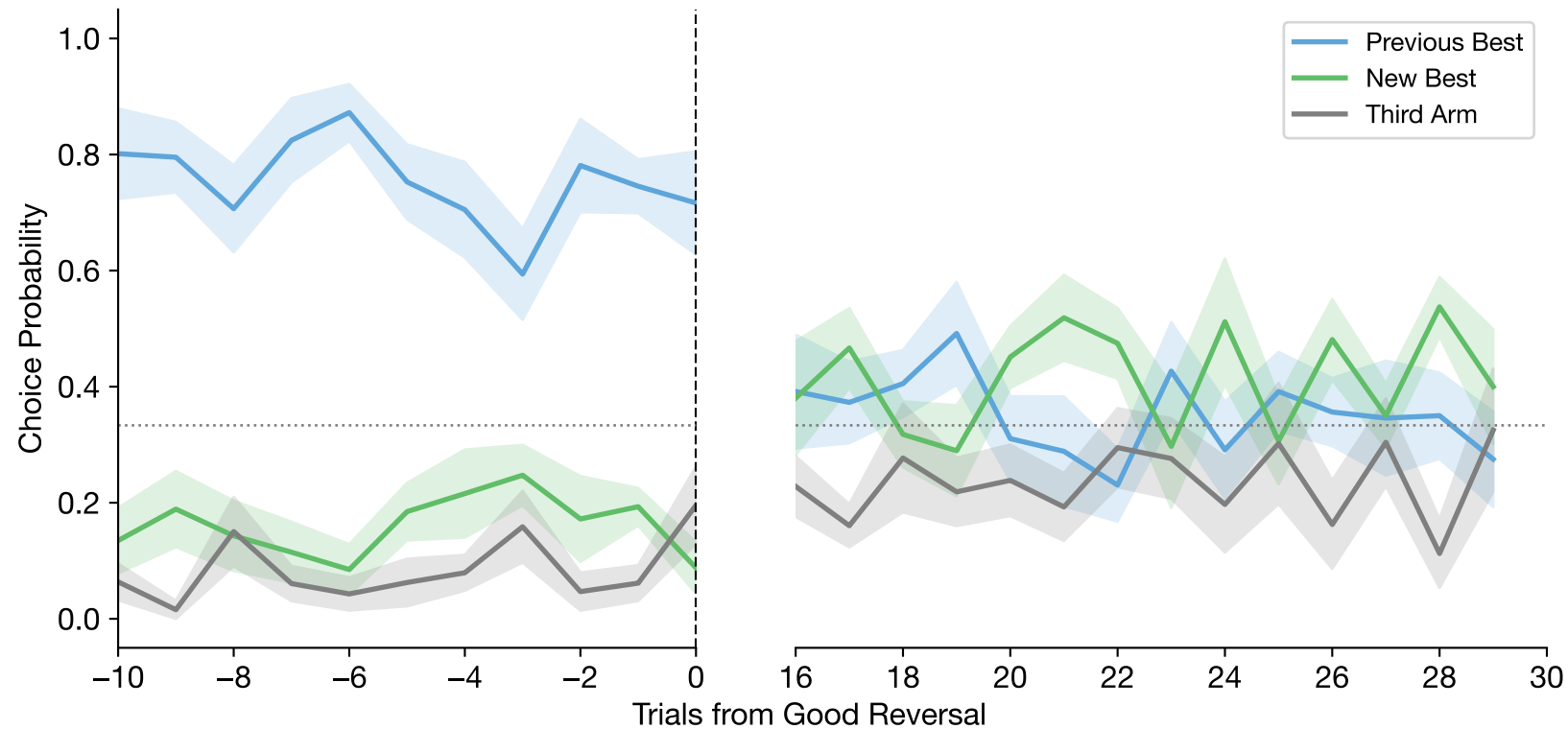
Good Reversal-Aligned Choices (mean \pm se across subjects | n=8 subjects, n=45 reversals) (Skipping first 15 trials post-reversal)
